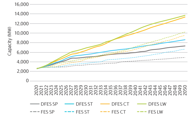
Figure 28 | Distributed generation and storage capacity comparison (Gen_BB001 to Gen_BB023, Srg_BB001 to Srg_BB004)
