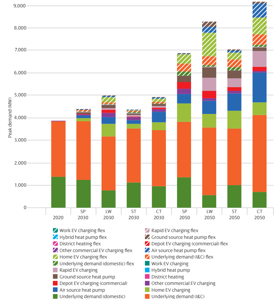
Figure 6 | Electricity peak demand breakdown for 2030 and 2050
