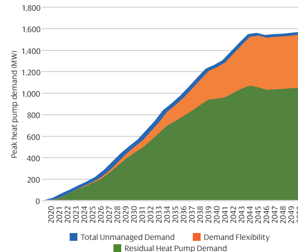
Figure 13 | Heat pump contribution to peak demand (high scenario)
