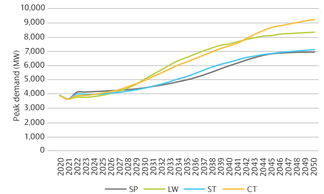
Figure 4 | Electricity peak demand without flexibility
