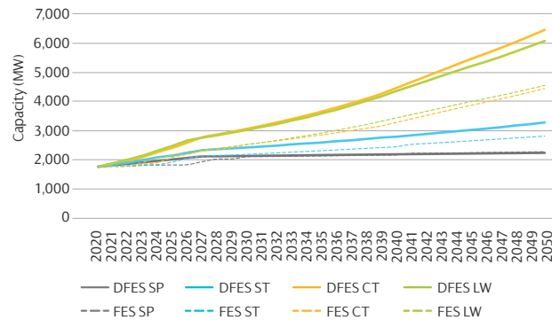
Figure 30 | Wind generation capacity comparison (Gen_BB014, Gen_BB015 and Gen_BB016)
