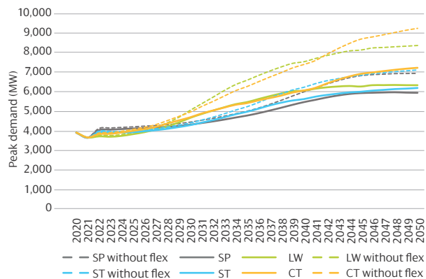
Figure 5 | Electricity peak demand with and without flexibility
