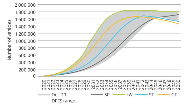
Figure 8 | Residential battery electric vehicle uptake
