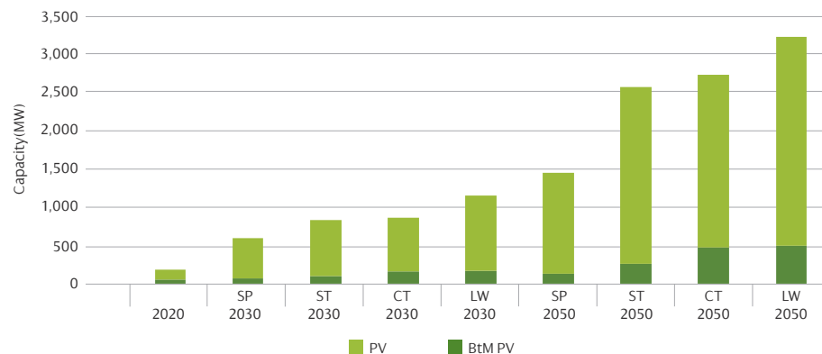
Figure 22 | Distribution connected and behind the meter solar PV capacity
