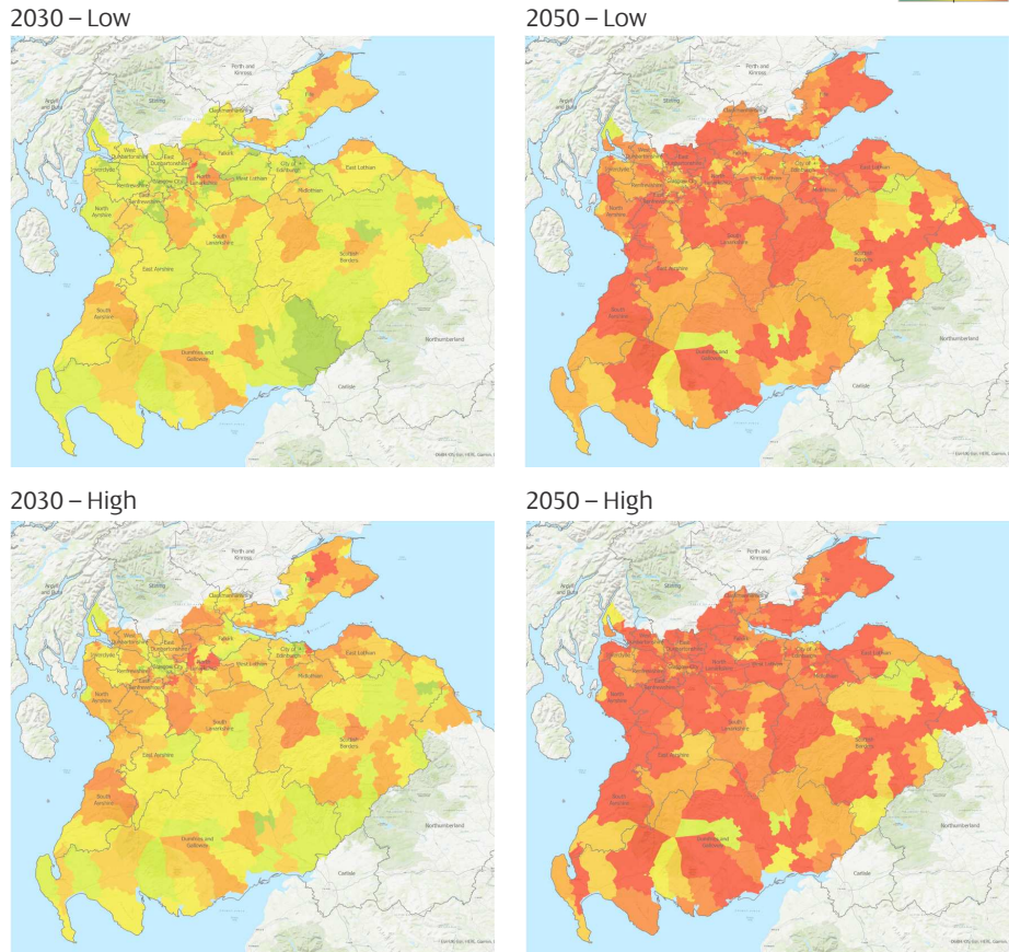
Figure 7 | Electricity peak demand changes from 2020 by primary substation area Scale range: -2MW to >10MW
