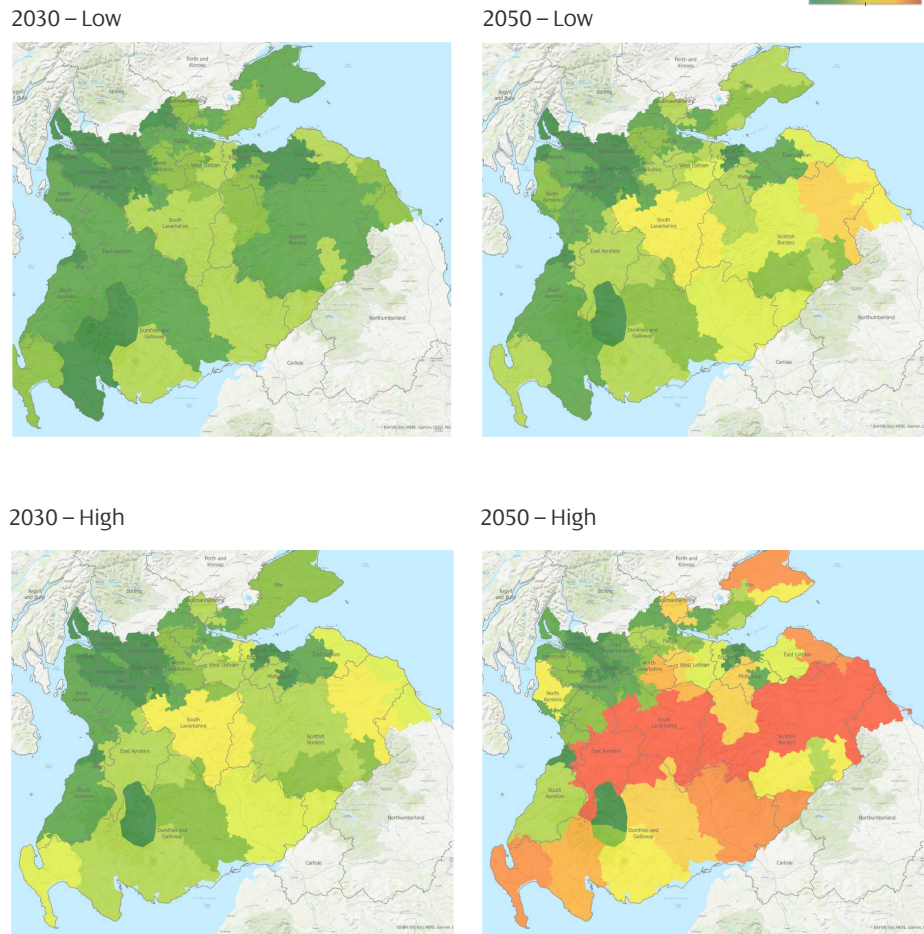
Figure 19 | Installed generation and storage capacity by GSP area Scale range: 0MW to >500MW
