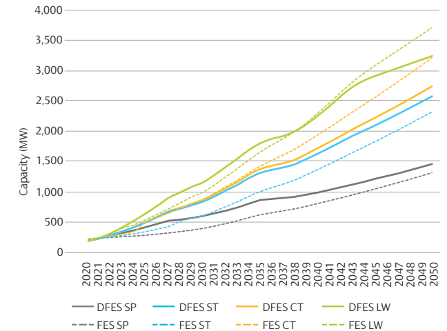
Figure 29 | Solar PV generation capacity comparison (Gen_BB012 and Gen_BB013)
