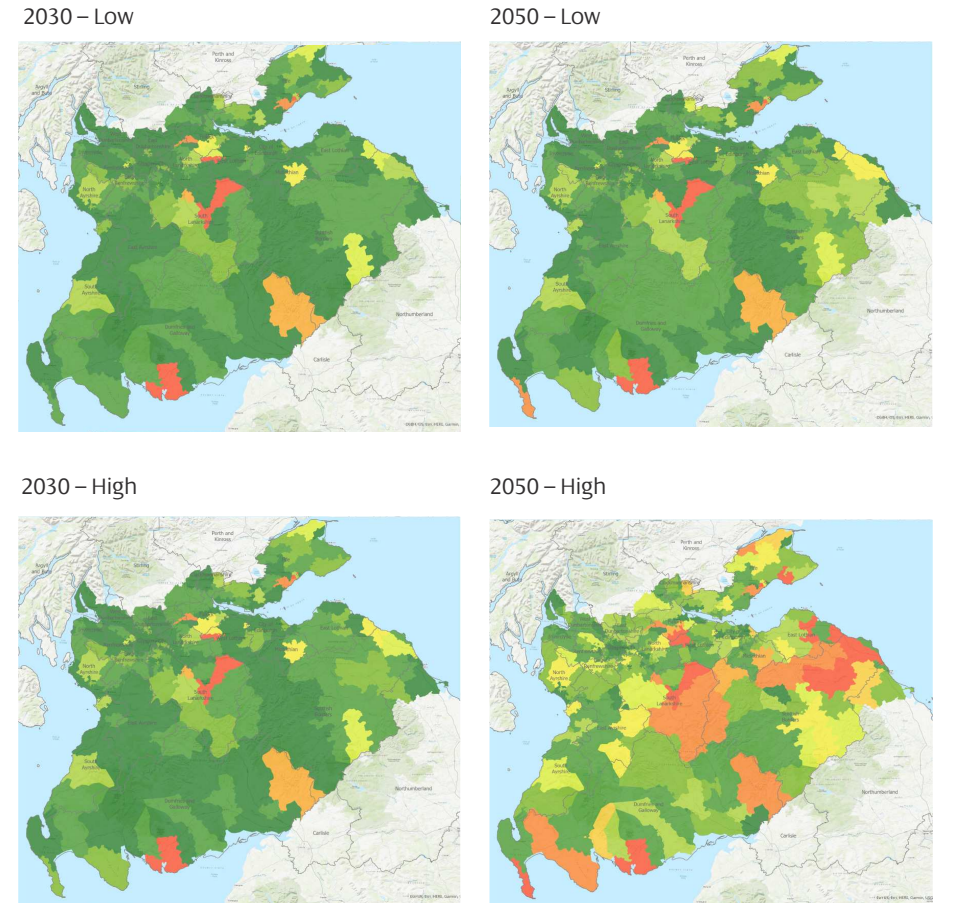
Figure 20 | Domestic-scale and smaller-scale installed generation and storage capacity by primary substation area Scale range: 0MW to >20MW
